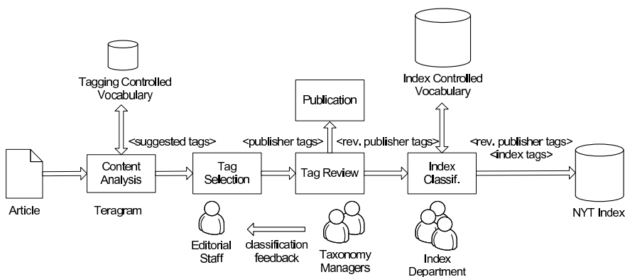
Fig. 1 The NYT article classification curation workflow
